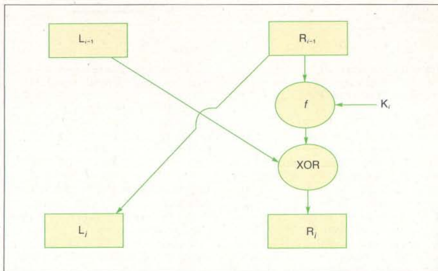
Figure 3: The details that are involved in each of the 16 rounds of encipherment shown in figure 2. Note that the new L part is the R part from the previous round, and the new R is the L part from the previous round XORed with the result of cipherfunction f .
